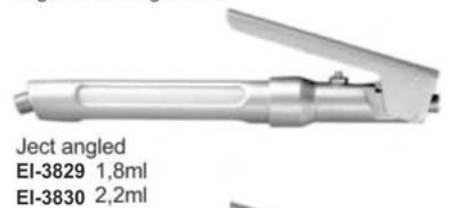
Ject Ultima EI-3823 1,8ml EI-3824 2,2ml Injects 0,05 ml with every click Supplied with angled and straight tubes
