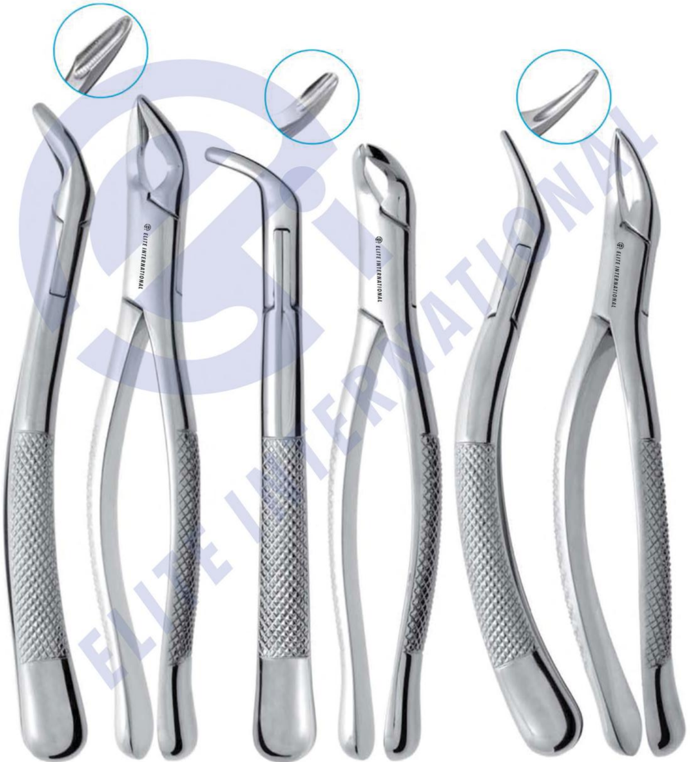
EI-3727 COHEN universal
